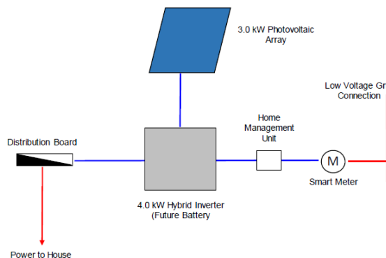
Figure: Photovoltaic Schematic
