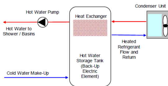
Figure: Hot Water Air Source Heat Pump Schematic
