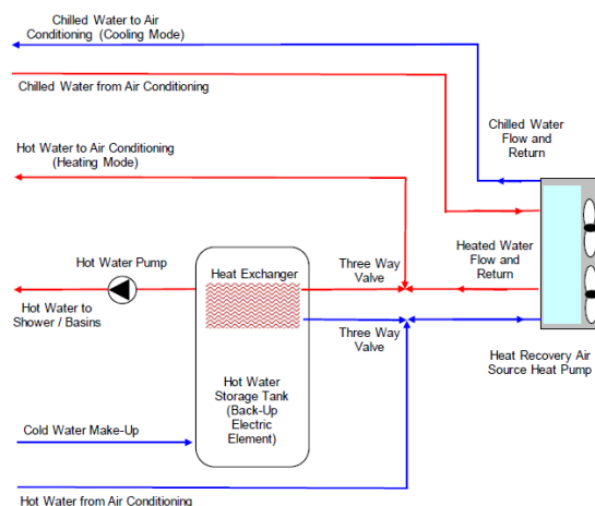
Figure: Heat Recovery Air Source Heat Pump Schematic
