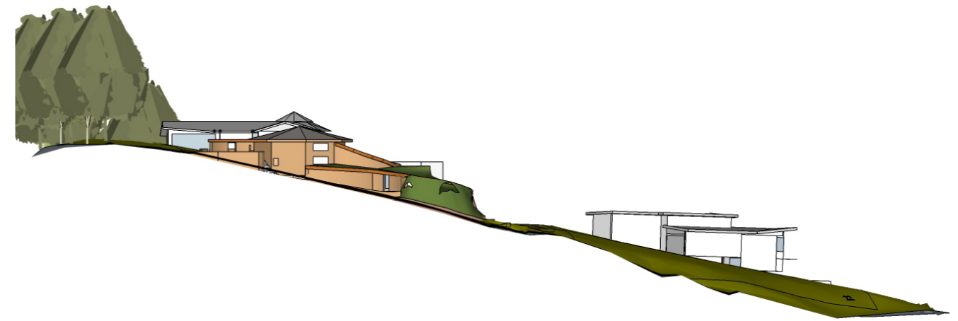
Elevation 5 – Building Envelope Lots 33 & 22
