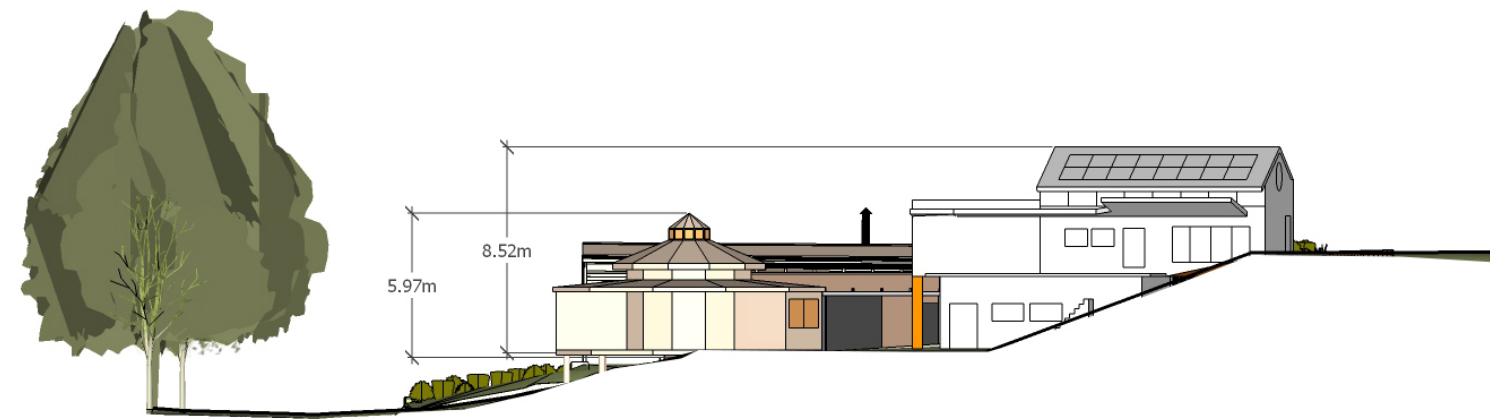
Elevation 3 – Building Envelope Lots 4-2
