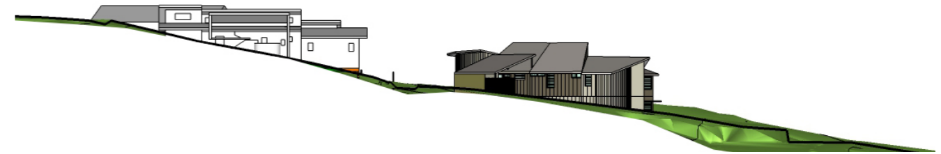
Elevation 5 – Building Envelope Lots 20 & 11
